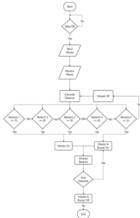
Fig 3: Flow chart System
