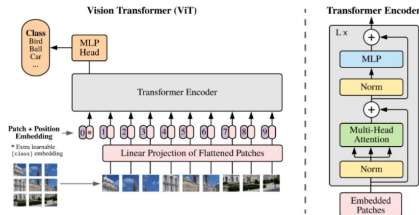
Figure 1. Vision Transformer (ViT) Architecture[25]
