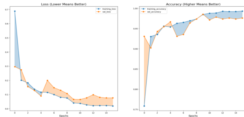
Figure 9. ViT_B16 Loss and Accuracy Graph on the First Dataset
