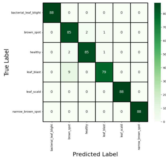
Figure 10. Confusion Matrix of First Dataset
