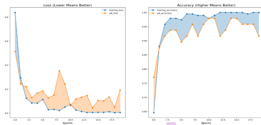
Figure 11. ViT_B16 Loss and Accuracy Graph on the Second Dataset
