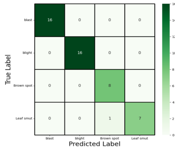
Figure 12. Confusion Matrix on the Second Dataset
