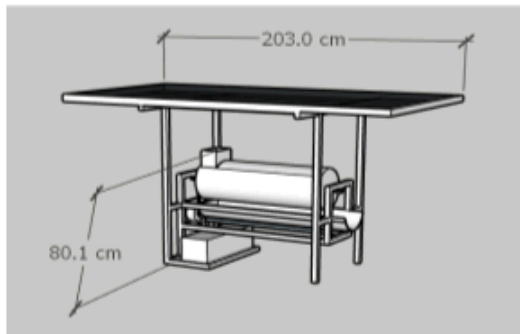
Figure 12. Design of the Corn Sheller Machine
