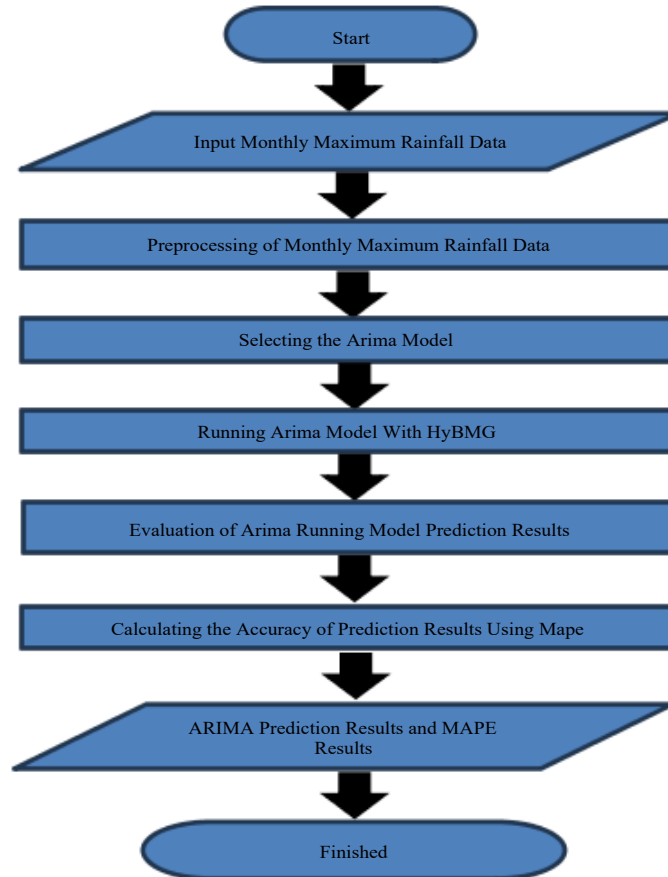
Fig. 1 Flowchart of ARIMA and processing algorithms MAPE
