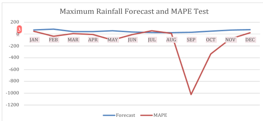
Fig 3. Maximum Rainfall Forecast and MAPE Test
