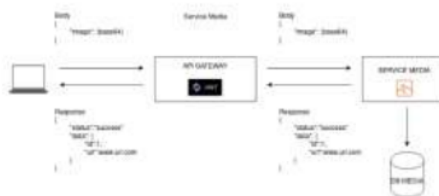
Gambar 6 Flow Service Media
