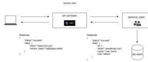
Gambar 4 Flow Service User
