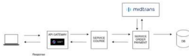
Gambar 9 Flow Service Order Payment
